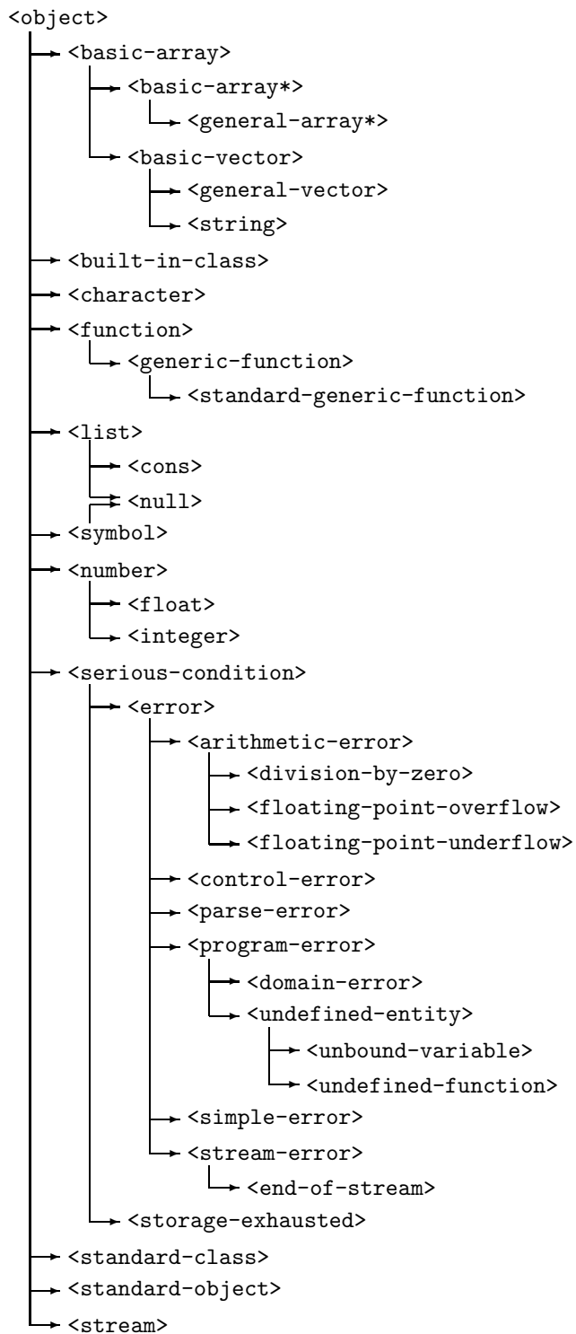
Figure 1. Class Inheritance
